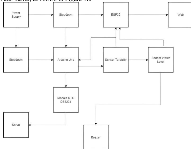
Figure 16. Block diagram
